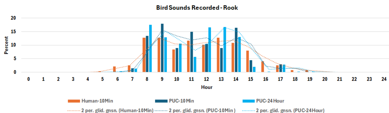
Figure 2. The percentage of recorded Rook sounds in each hour for a human listener in 10 minutes per hour (red), a BirdWeather PUC in 10 minutes per hour (dark blue) and a BirdWeather PUC in 24 hours (light blue). Running averages are shown as dotted lines.
