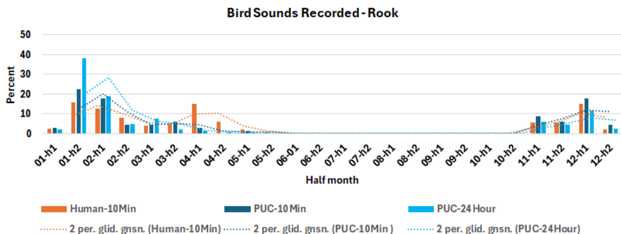
Figure 4. The percentage of recorded Rook sounds in each half month for a human listener in 10 minutes per hour (red), a BirdWeather PUC in 10 minutes per hour (dark blue) and a BirdWeather PUC in 24 hours (light blue). Running averages are shown as dotted lines.
