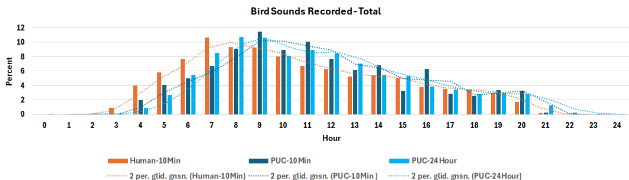
Figure 1. The percentage of recorded bird sounds of all species in each hour for human listener in 10 minutes per hour (red), a BirdWeather PUC in 10 minutes per hour (dark blue) and a BirdWeather PUC in 24 hours (light blue). Running averages are shown as dotted lines.
