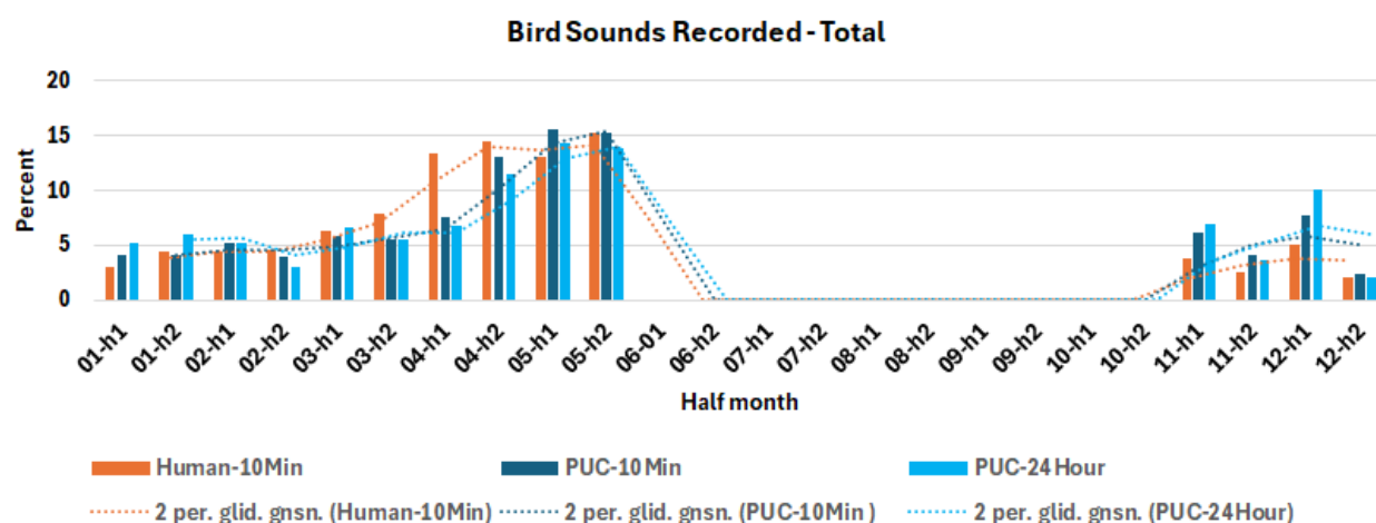
Figure 3. The percentage of recorded bird sounds of all species in each half-month for a human listener in 10 minutes per hour (red), a BirdWeather PUC in 10 minutes per hour (dark blue) and a BirdWeather PUC in 24 hours (light blue). Running averages are shown as dotted lines.
